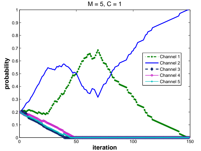
Fig. 3. The probability updating history of the stochastic channel selection algorithm.
